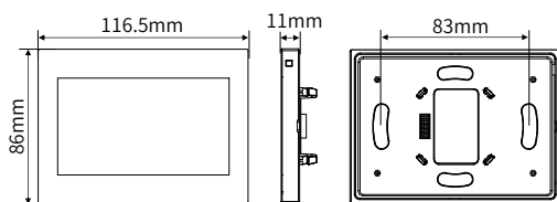
Figure 6. Dimensions - Front View Figure 7. Side View Figure 8. Back View
