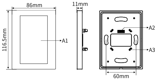
Figure 2. Dimensions - Front View Figure 3. Side View Figure 4. Back View
