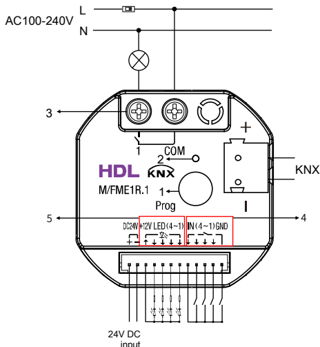
Figure 7. Wiring
