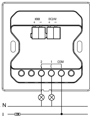
Figure 7. Wiring
