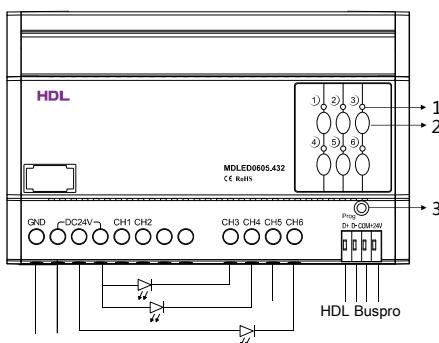
Figure 4. Wiring
