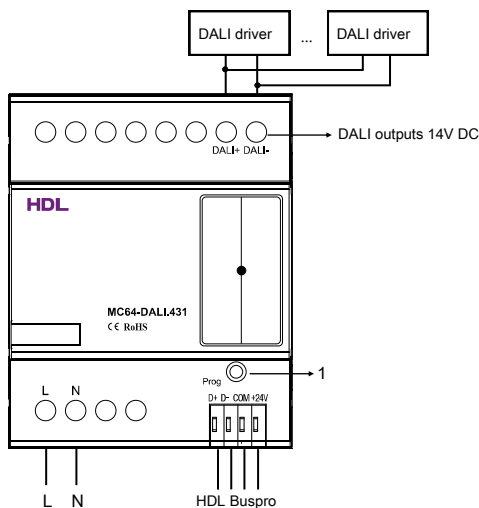
Figure 4. Wiring
