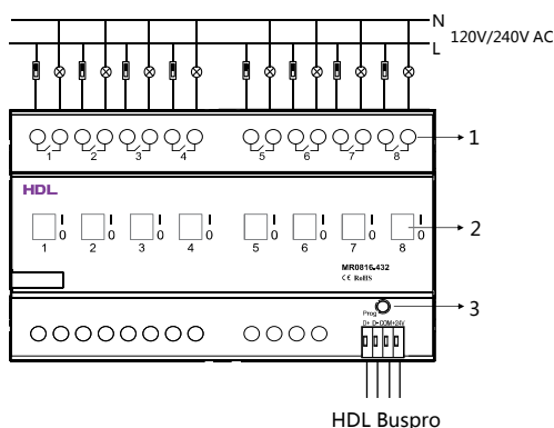
Figure 4. Wiring
