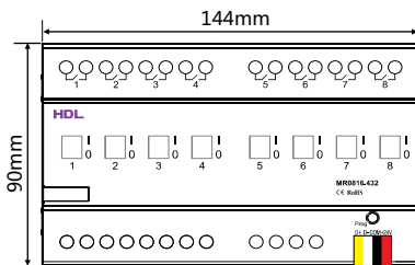
Figure 2. Dimensions - Front View
