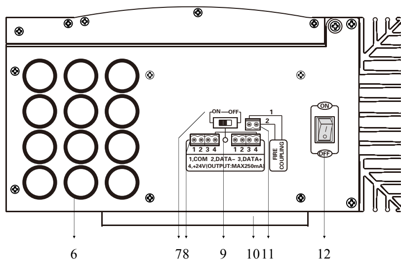
Underside
