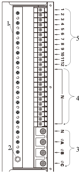
Power input and load wiring terminal
