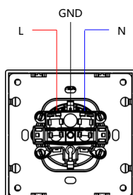
Figure 4. Wiring
