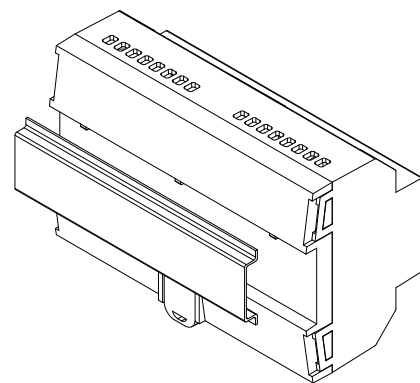
Figure 2: Mounting MAXinBOX 16 v4 on DIN rail
