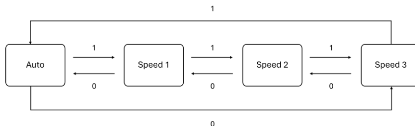
Figure 7. Cyclical fan step control (three fan speeds with automatic mode)
