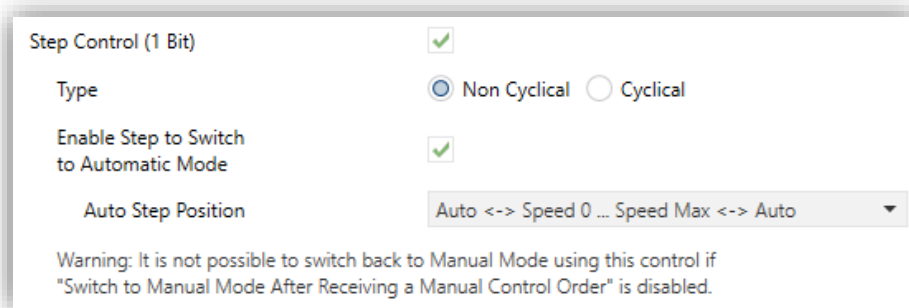
Figure 17 Fan Speed 1-Bit Step Control
