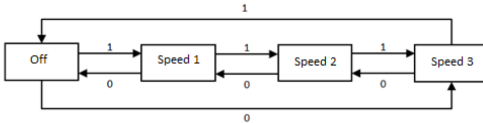
Figure 16. Cyclical fan step control. (with three fan speeds).
