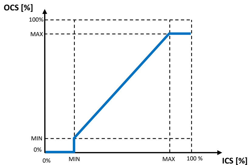
Figure 11. Fan Coil – Control signal scaling.
