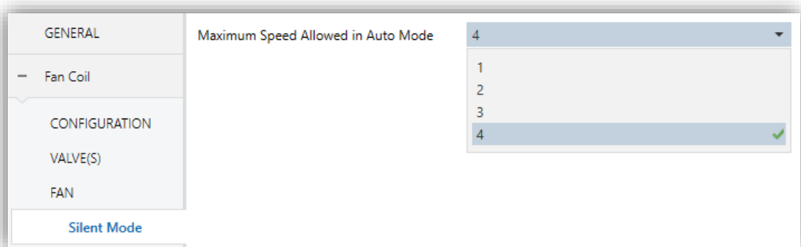
Figure 19. Fan Coil – Silent Mode
