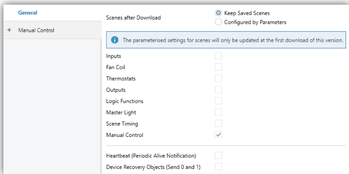
Figure 1 General screen.
